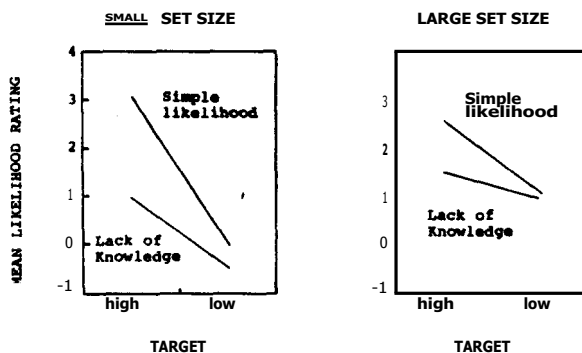
Figure 2. Results of Experiment 2: Mean ratings of the likelihood of target assertions of high or low importance for both the simple likelihood condition and the lack-of-knowledge condition, in the context of either a small set or a large set of similar assertions.
