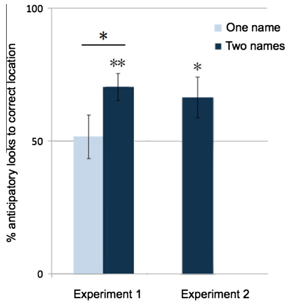
Fig. 4. Mean anticipatory looking to the correct door in each condition.
